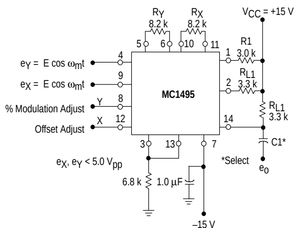
Figure 30. Amplitude Modulation
