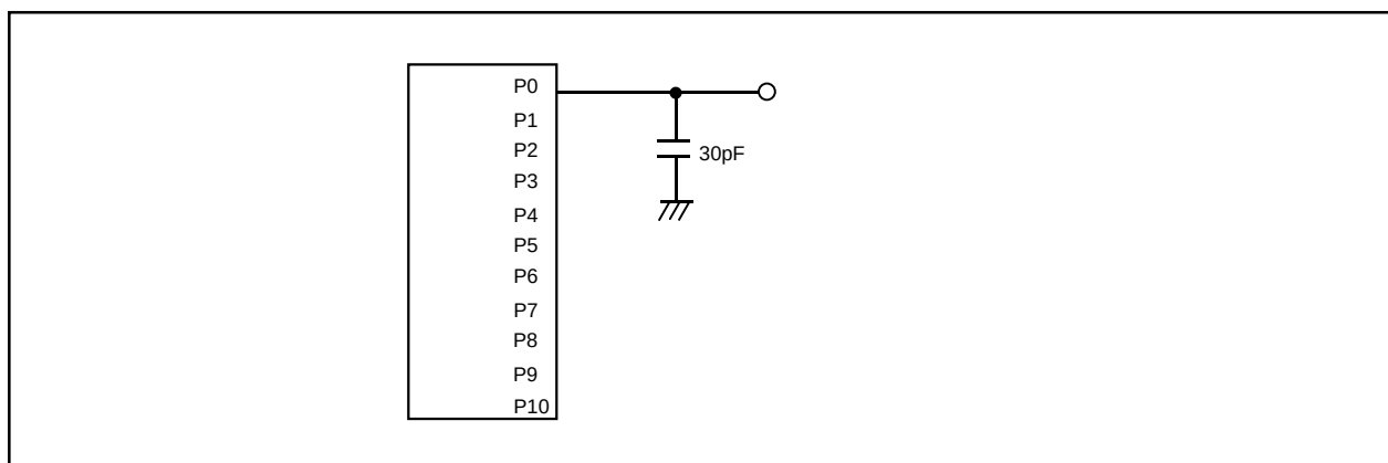
Figure 1.31.1. Port P0 to P10 measurement circuit
