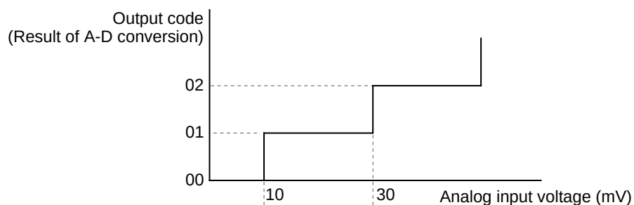
Optimal conversion characteristics in 8-bit mode ( V_{REF} = 5.12 \text{ V} )
