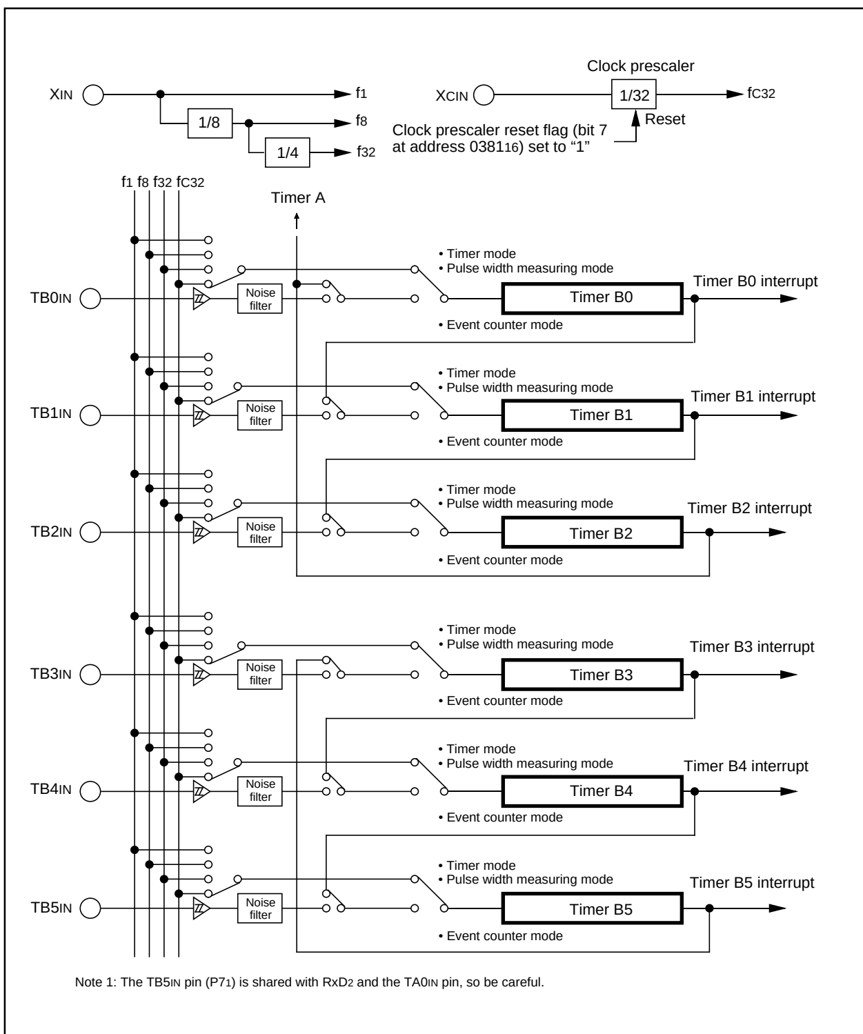
Figure 1.14.2. Timer B block diagram
