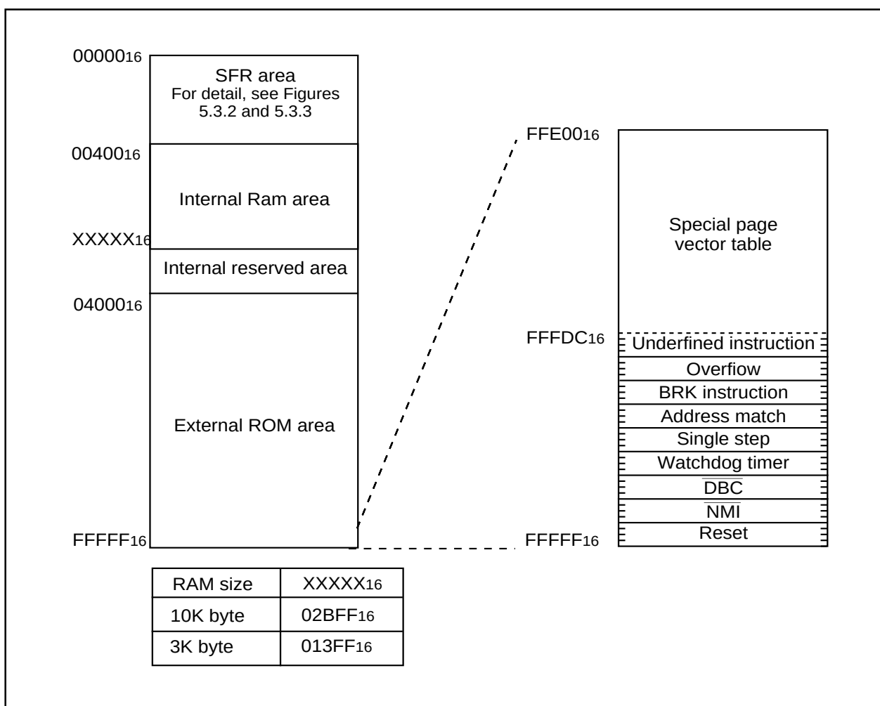
Figure 5.3.1. Memory map
