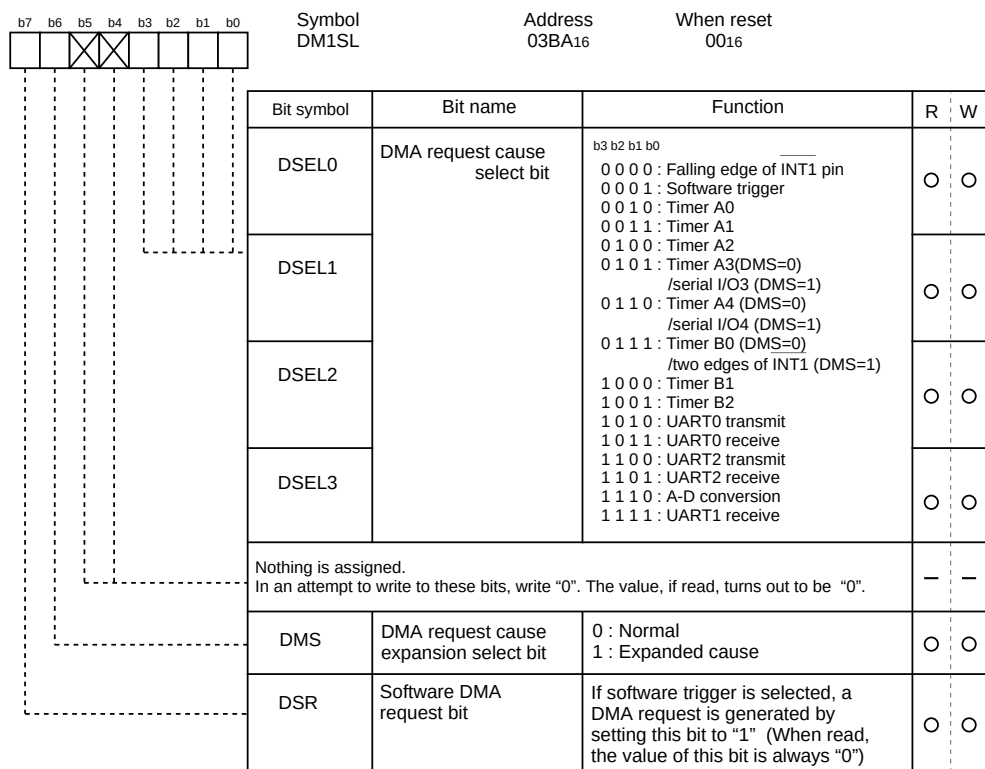
Figure 2.9.2. DMAC-related registers (1)
