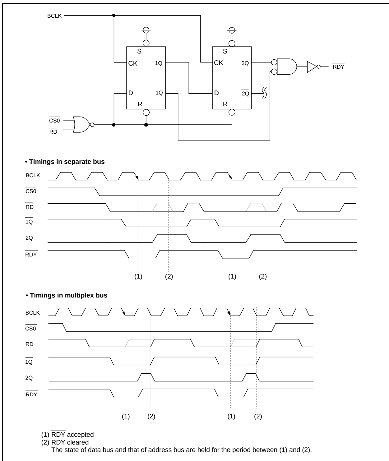
Figure 4.4.6. Example of \overline{\text{RDY}} circuit holding state of bus for 1 BCLK
