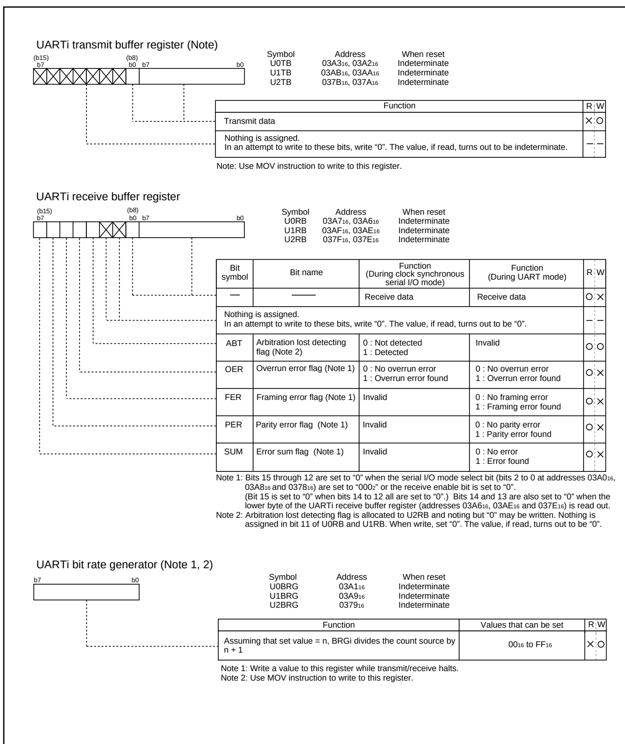
Figure 2.5.3. UARTi-related registers (1)
