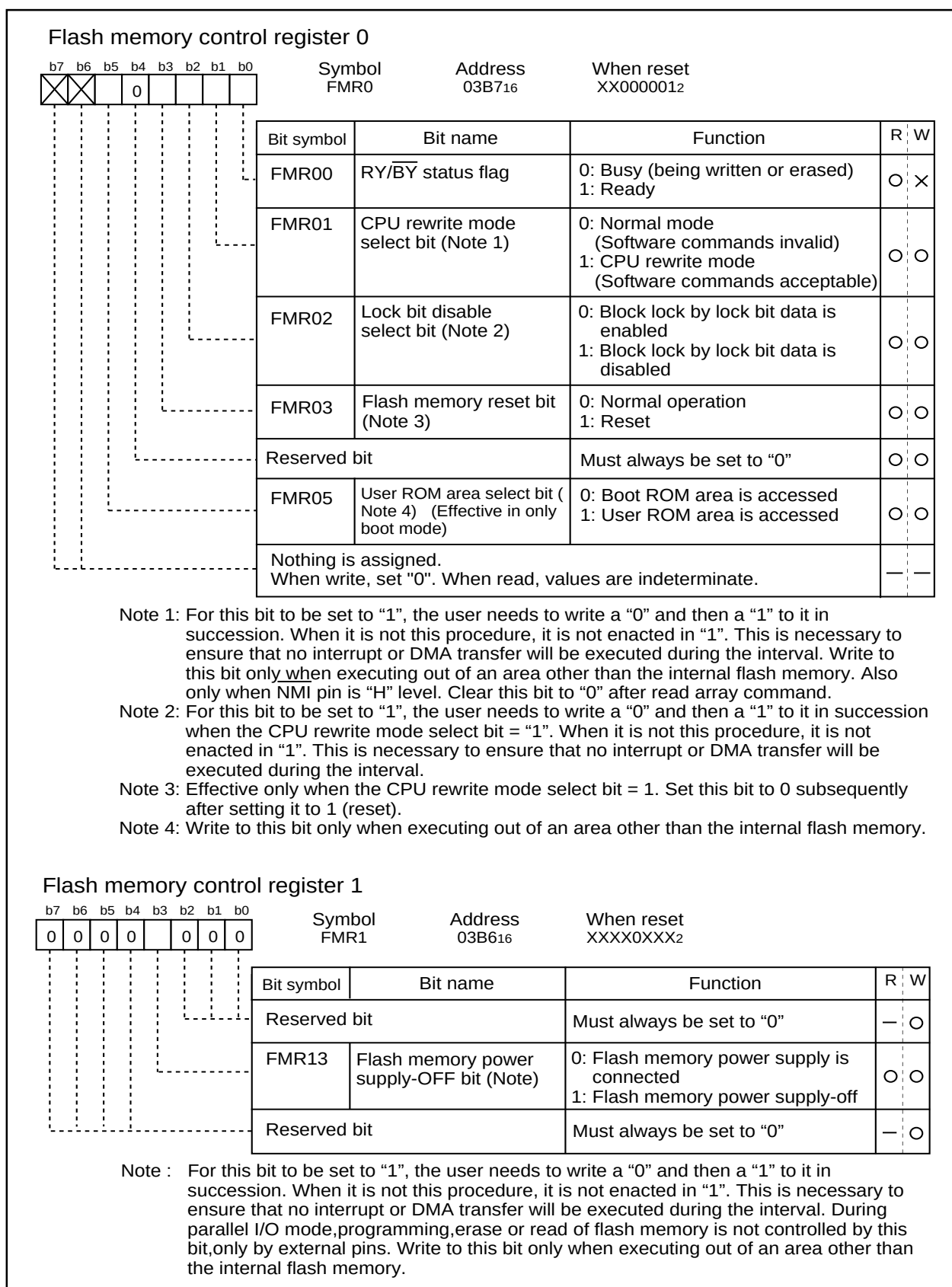
Figure 1.26.1. Flash memory control registers
