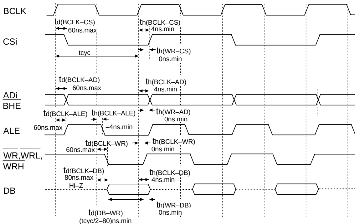
Figure 1.31.4. V CC =3V timing diagram (3)
