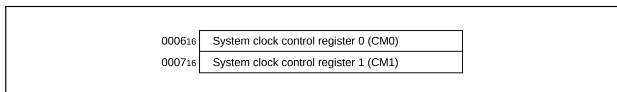
Figure 2.15.3. Memory map of power control-related registers
