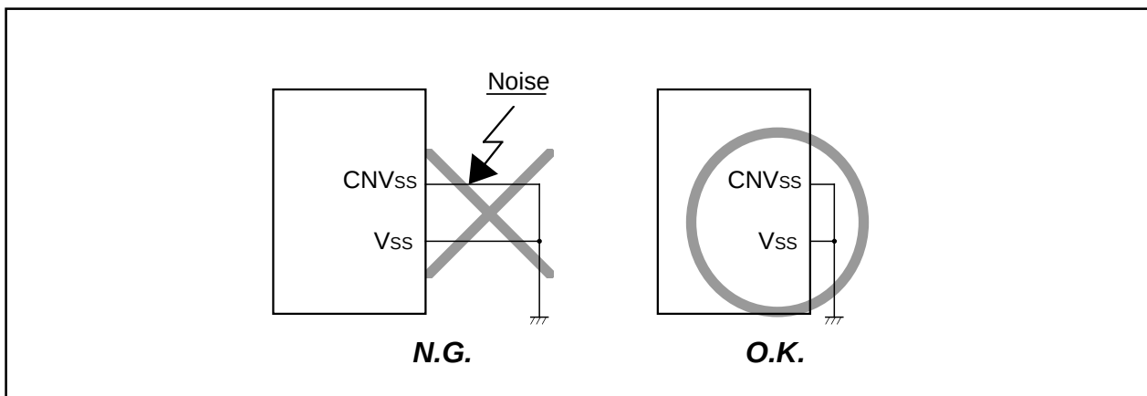
Figure 1.1.4. Wiring for CNVss pin
