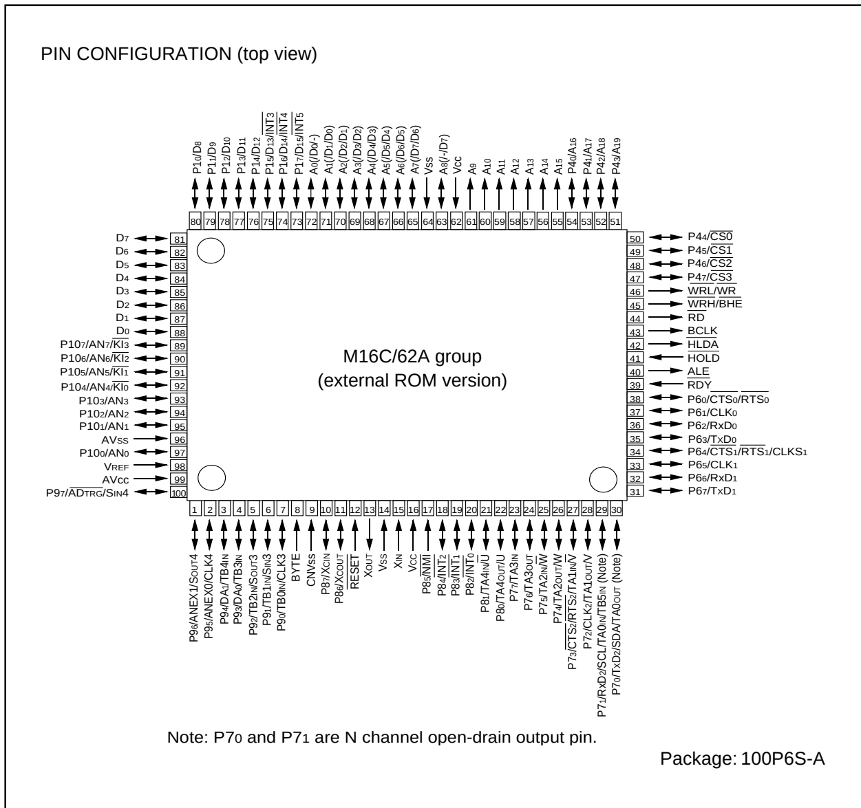
Figure 5.1.1. Pin configuration (top view)
