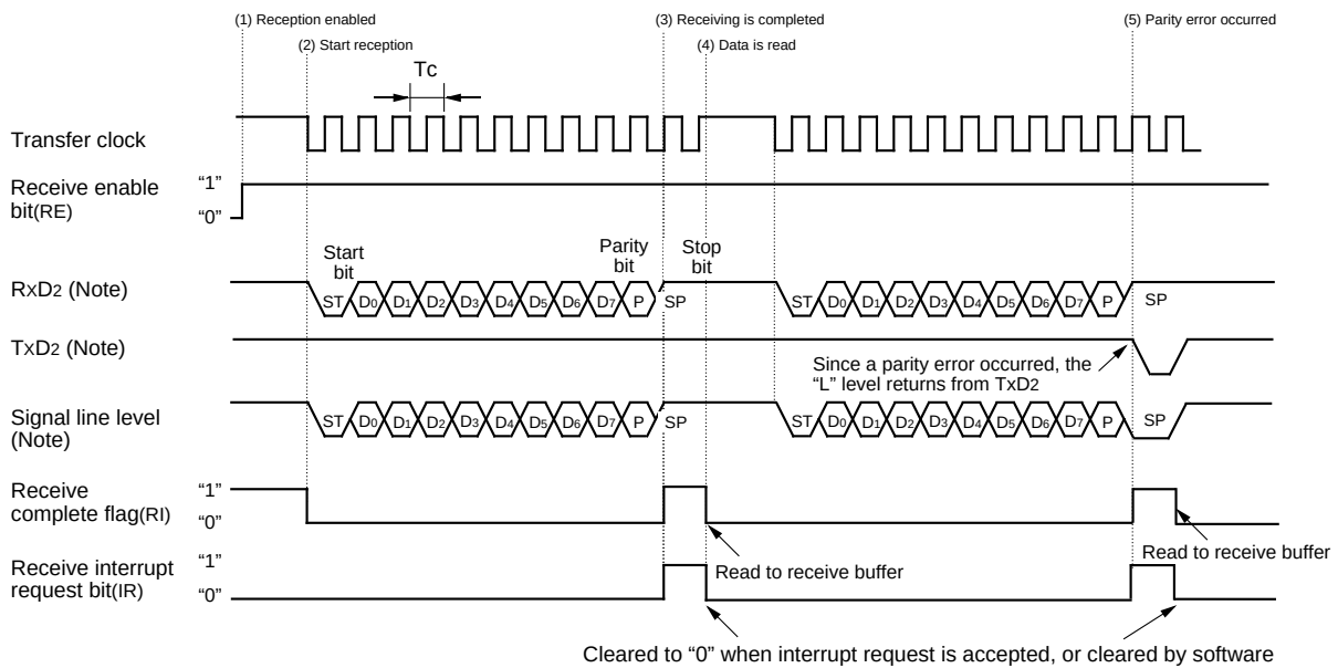
Figure 2.5.17. Operation timing of reception in UART mode (used for SIM interface)
