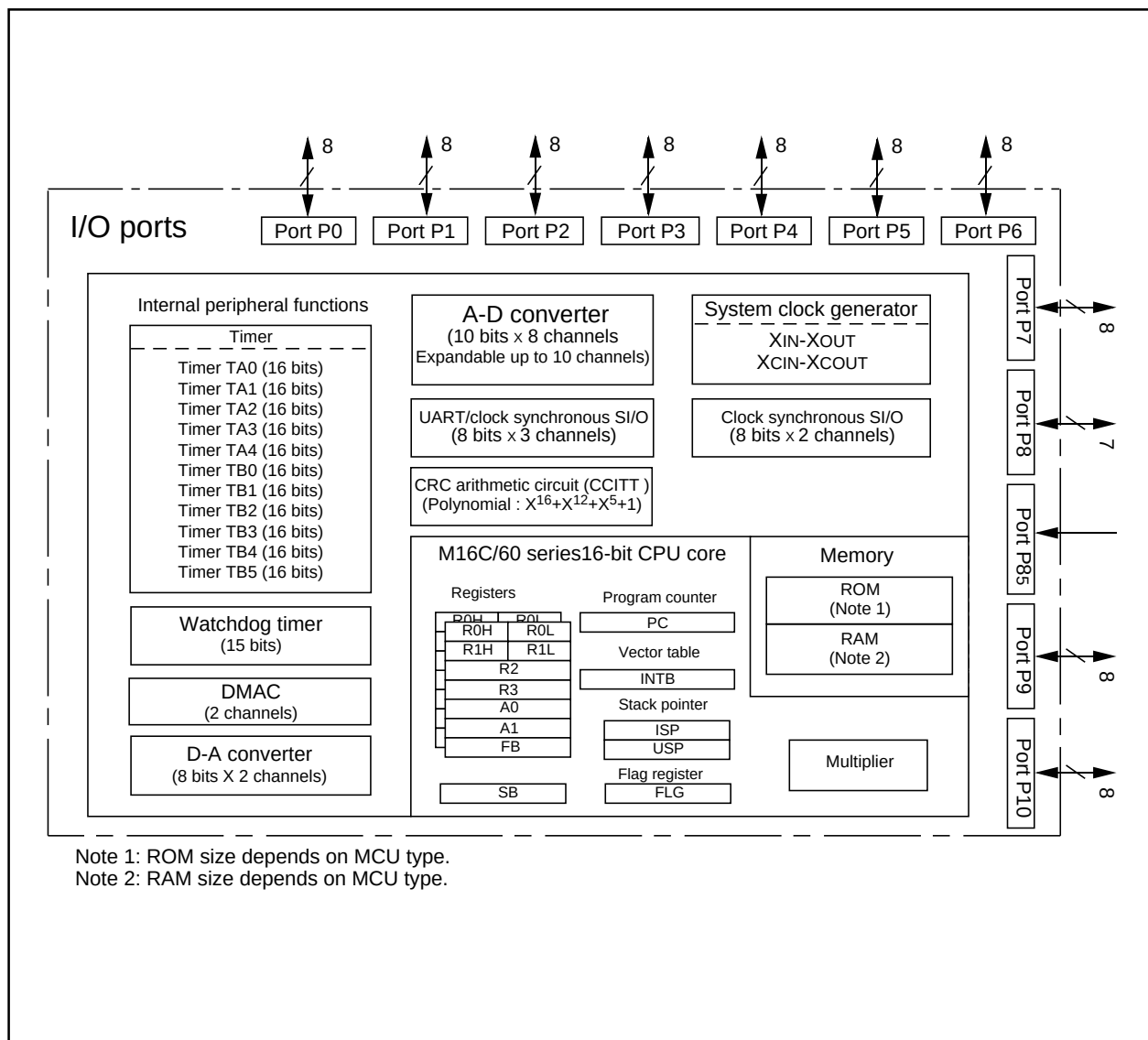
Figure 1.30.3. Block diagram of M16C/62M group
