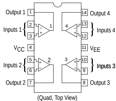
DTB SUFFIX PLASTIC PACKAGE CASE 751A (TSSOP-14)
