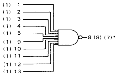
MC1804/MC1904 MC1805/MC1905 10-Input NAND Gate
