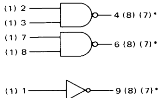
MC862G/MC962G MC863G/MC963G Dual 2-Input NAND Gate Plus Inverter
