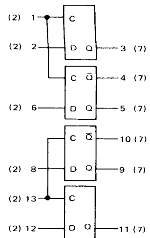
MC1814/MC1914 Quad Latch
