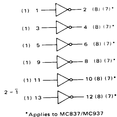
MC836/MC936 MC837/MC937 Hex Inverter
