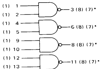
MC846/MC946 MC849/MC949 Quad 2-Input NAND Gate
