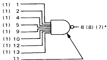
MC1802/MC1902 MC1803/MC1903 Expandable 8-Input NAND Gate
