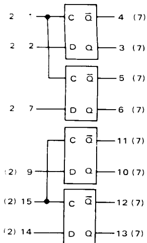
MC1813 Quad Latch
