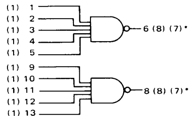
MC1800/MC1900 MC1801/MC1901 Dual 5-Input NAND Gate
