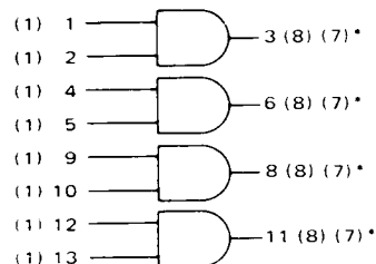
MC1806/MC1906 MC1807/MC1907 Quad 2-Input AND Gate
