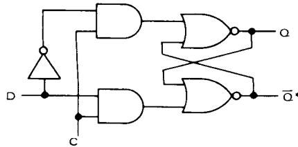
FUNCTIONAL LOGIC DIAGRAM
