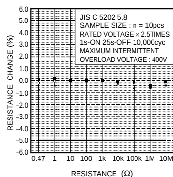
Fig.10 Intermittent overload
