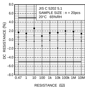
Fig.5 DC resistance
