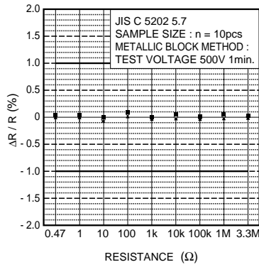
Fig.9 Withstand voltage
