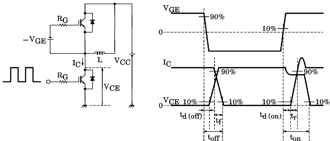
(Note 1) Switching Time Test Circuit & Timing Chart
