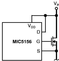
Figure 3. No Current Limit
