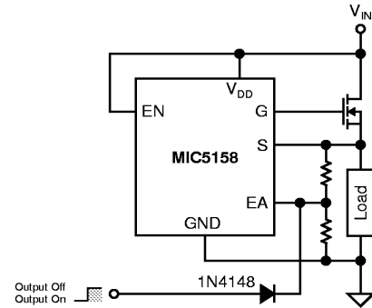
Figure 4b. Fast High-Side Switch
