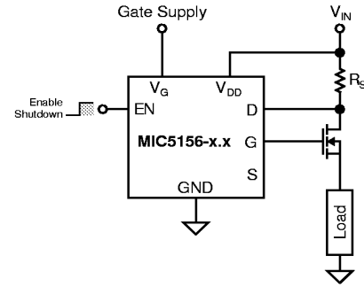
Figure 4a. High-Side Switch
