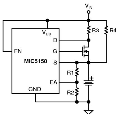
Figure 5. Battery Charger Concept
