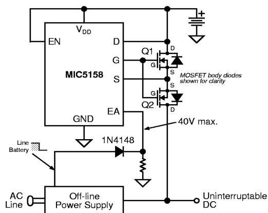
Figure 6. UPS Power Supply Concept
