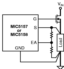
Figure 1b. Connections for Adjustable Output
