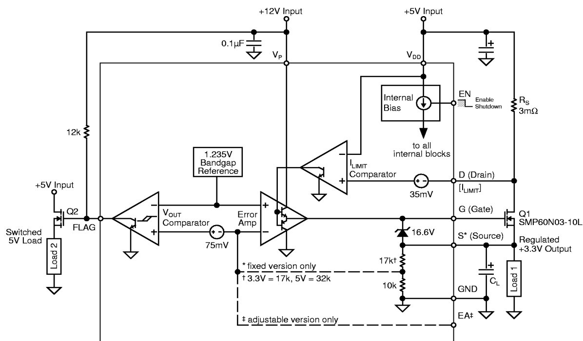
Block Diagram with External Components Fixed 3.3V Power Supply with 5.0V Load Switch
