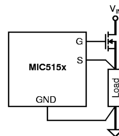
Figure 1a. Connections for Fixed Output
