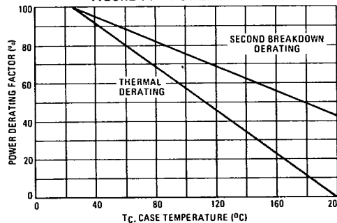
FIGURE 14 — POWER DERATING
