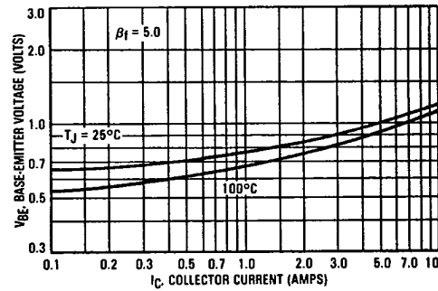
FIGURE 4 — BASE-EMITTER VOLTAGE
