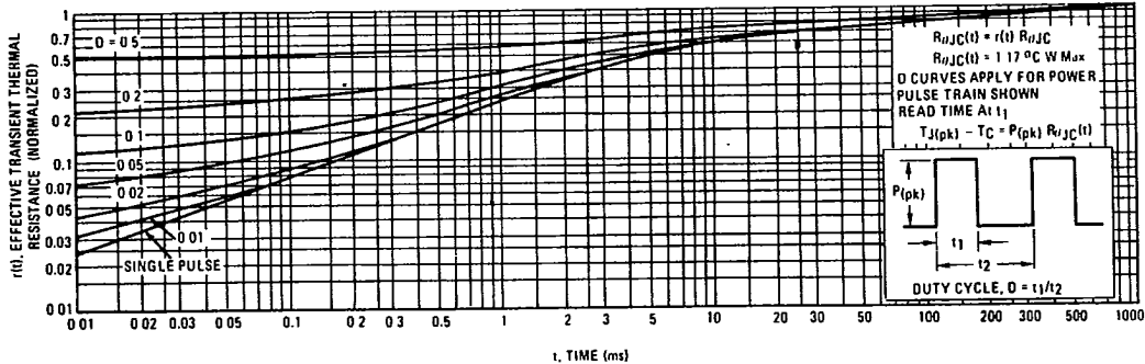
FIGURE 11 — THERMAL RESPONSE
