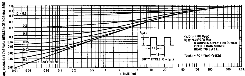
FIGURE 11 - THERMAL RESPONSE
