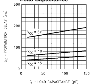
Propagation Delay, LATCH ENABLE to Output vs Load Capacitance
