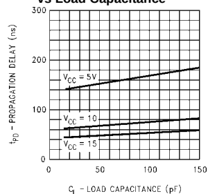
Propagation Delay, Data In to Output vs Load Capacitance
