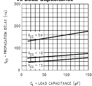
Propagation Delay, CLOCK to Output vs Load Capacitance
