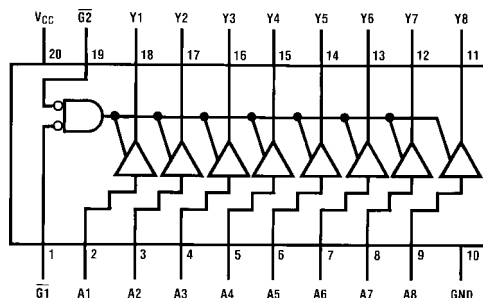
Top View MM74HCT541
