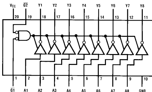
Top View MM74HCT540
