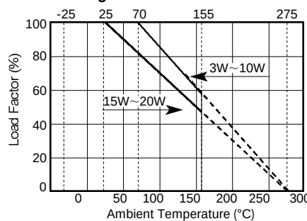
Derating Curve
