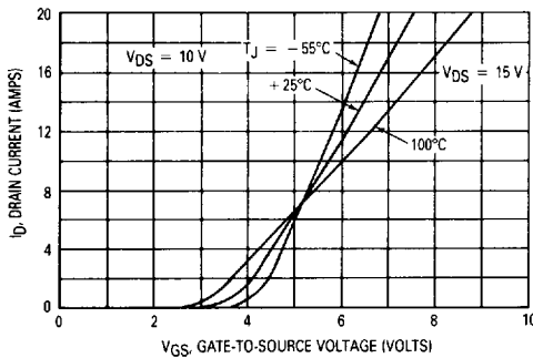
Figure 4. Transfer Characteristics
