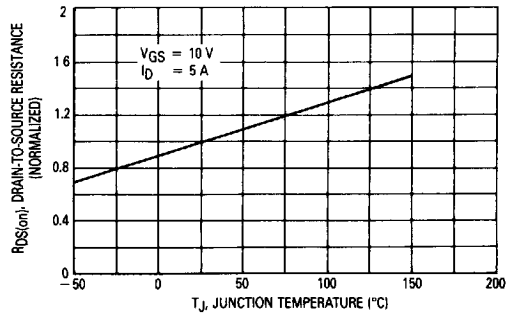
Figure 7. On-Resistance Variation With Temperature
