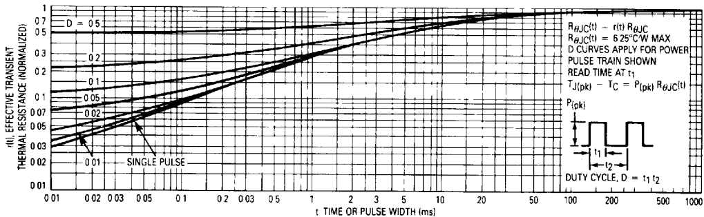
Figure 10. Thermal Response
