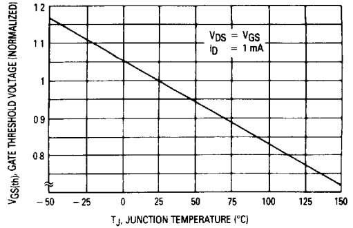
Figure 3. Gate-Threshold Voltage Variation With Temperature
