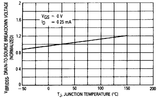
Figure 5. Breakdown Voltage Variation With Temperature
