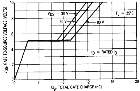
Figure 12. Gate Charge versus Gate-To-Source Voltage
