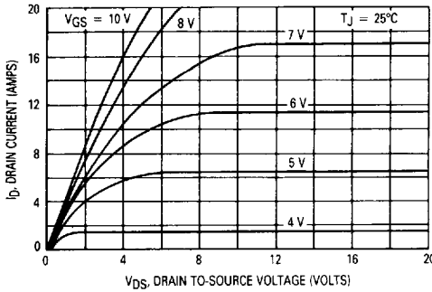
Figure 2. On-Region Characteristics
