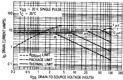
Figure 8. Maximum Rated Forward Biased Safe Operating Area
