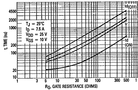
Figure 9. Resistive Switching Time Variation versus Gate Resistance
