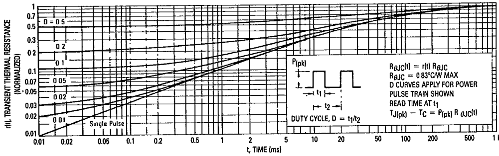
Figure 10. Thermal Response
