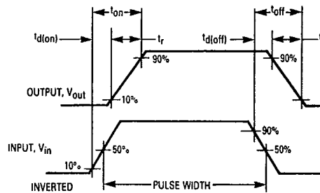
Figure 14. Switching Waveforms
