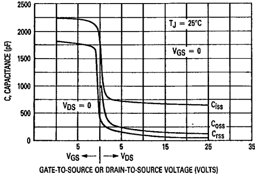
Figure 11. Capacitance Variation
