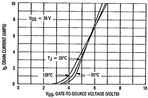
Figure 3. Transfer Characteristics
