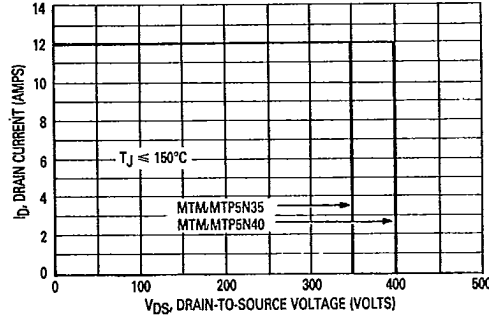
Figure 8. Maximum Rated Switching Safe Operating Area
