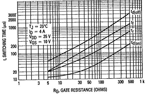
Figure 9. Resistive Switching Time Variation versus Gate Resistance
