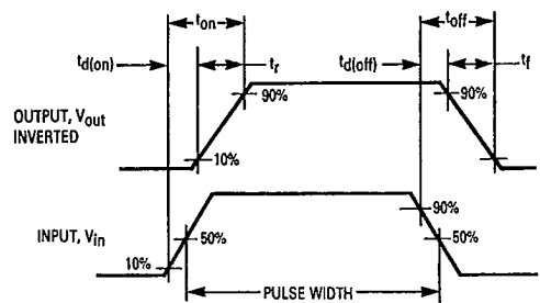
Figure 14. Switching Waveforms
