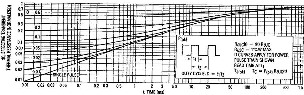
Figure 10. Thermal Response
