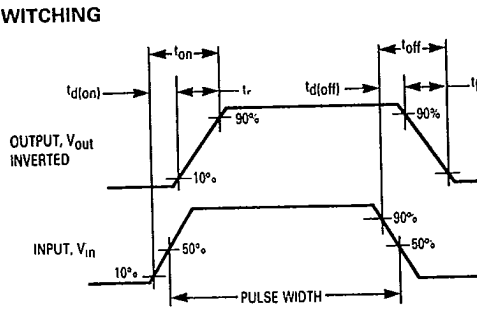
Figure 14. Switching Waveforms
