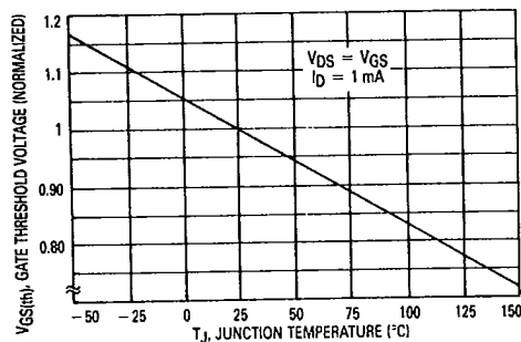
Figure 2. Gate-Threshold Voltage Variation With Temperature
