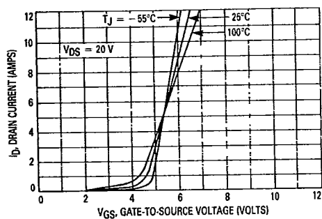
Figure 3. Transfer Characteristics
