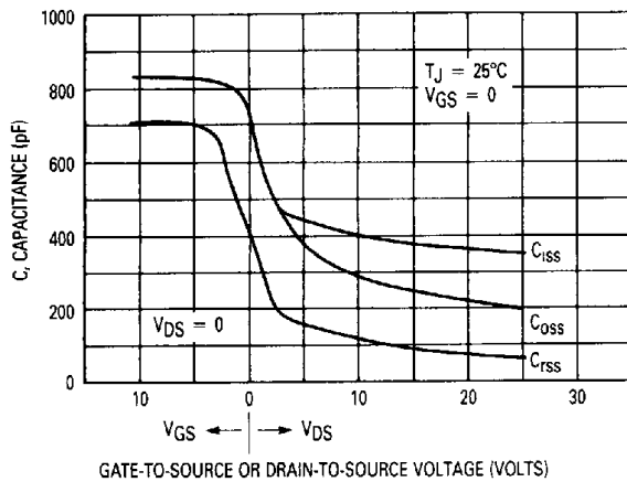
Figure 11. Capacitance Variation
