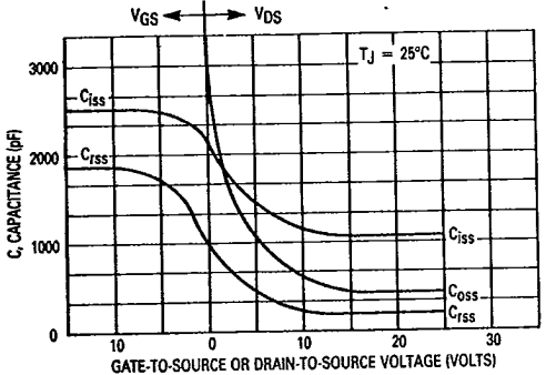
Figure 16. Capacitance Variation
