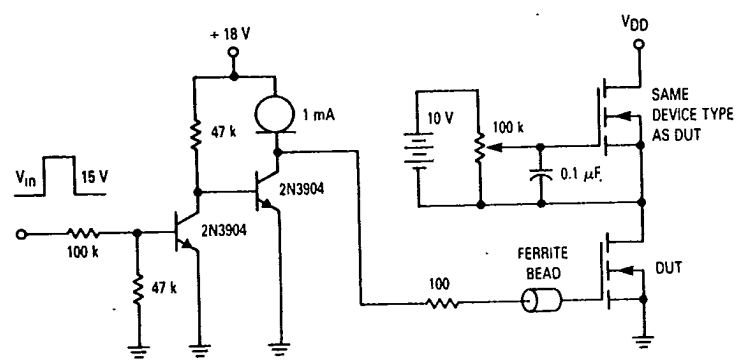
Figure 16. Capacitance Variation
