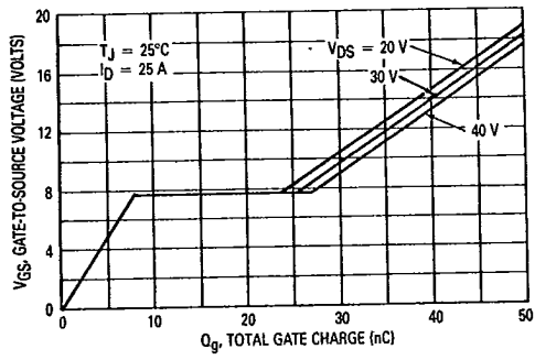
Figure 17. Gate Charge versus Gate-to-Source Voltage
