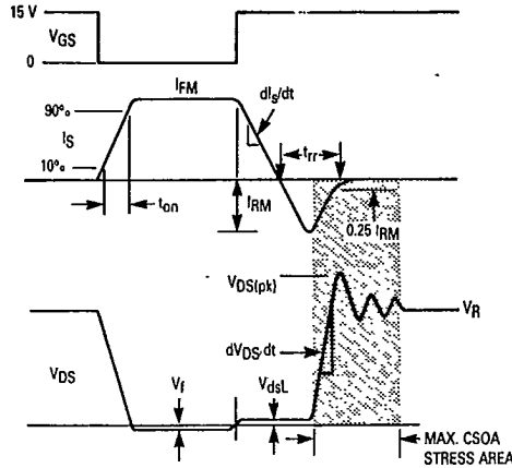
Figure 11. Commutating Waveforms
