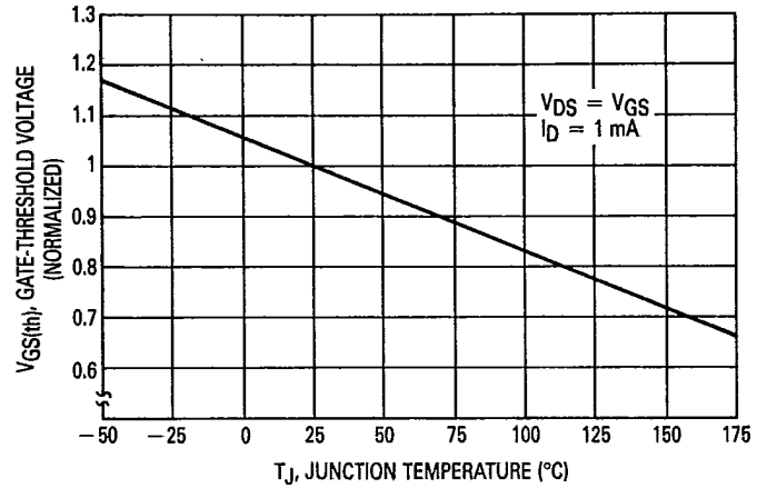
Figure 2. Gate-Threshold Voltage Variation With Temperature
