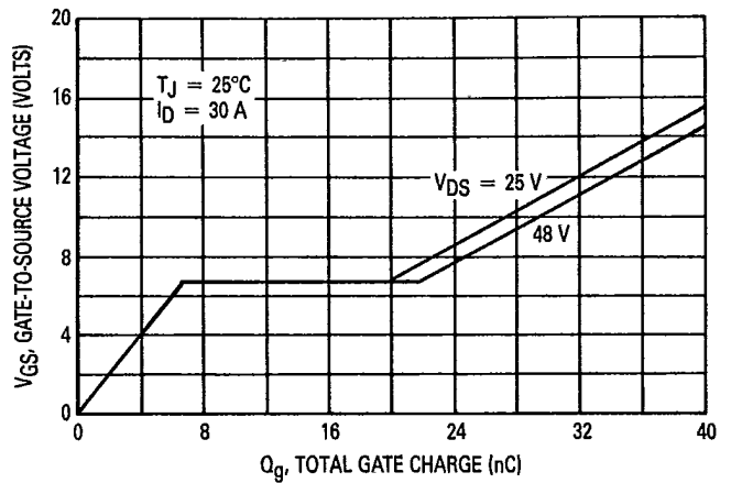
Figure 17. Gate Charge versus Gate-To-Source Voltage
