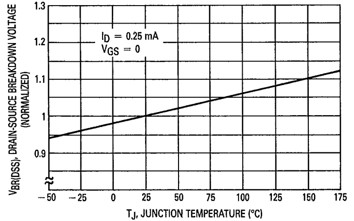
Figure 4. Breakdown Voltage Variation With Temperature
