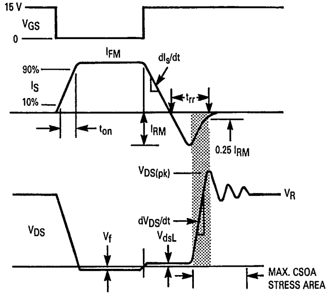
Figure 13. Commutating Safe Operating Area Test Circuit
