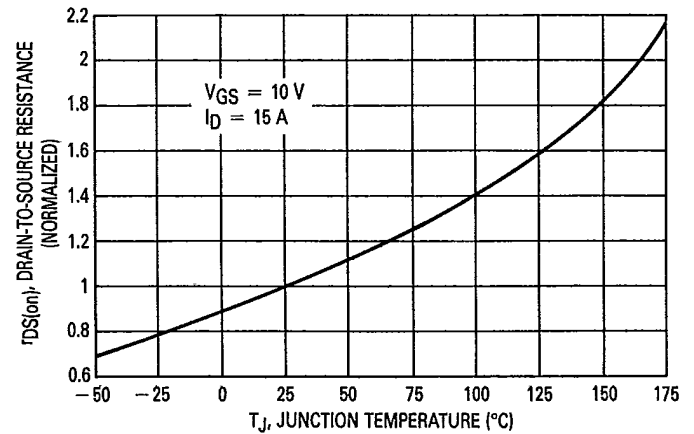
Figure 6. On-Resistance Variation With Temperature
