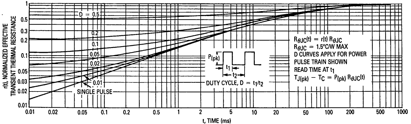
Figure 10. Thermal Response
