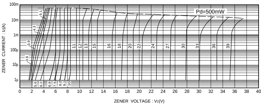
Fig.1 Zener characteristics
