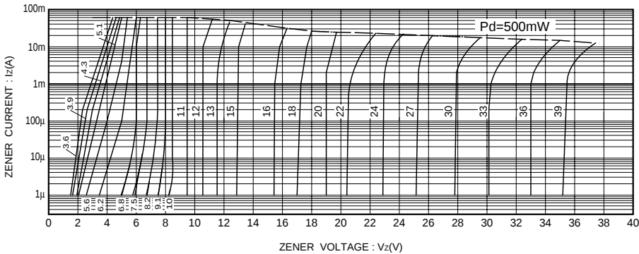
Fig.1 Zener characteristics
