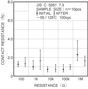
Fig.10-2 Temperature cycling
