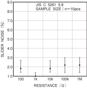
Fig.14 Wiper noise
