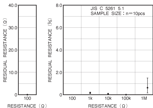
Fig.4 Residual resistance
