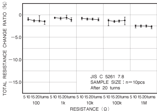
Fig.6-1 Endurance (wiper)
