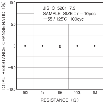
Fig.10-1 Temperature cycling
