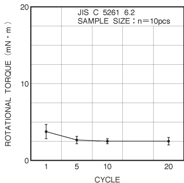
Fig.7 Rotational torque
