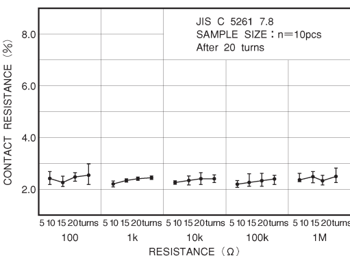
Fig.6-2 Endurance (wiper)
