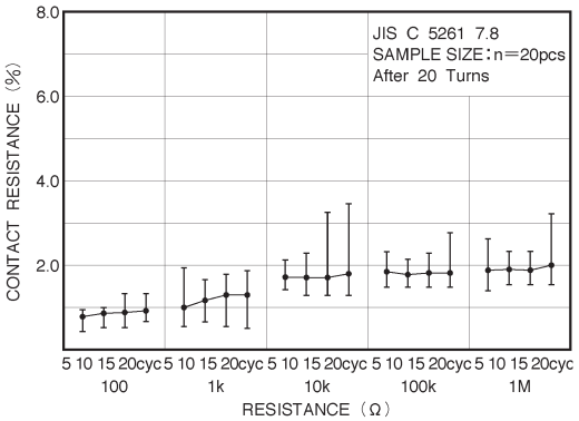
Fig.5-2 Endurance (wiper)
