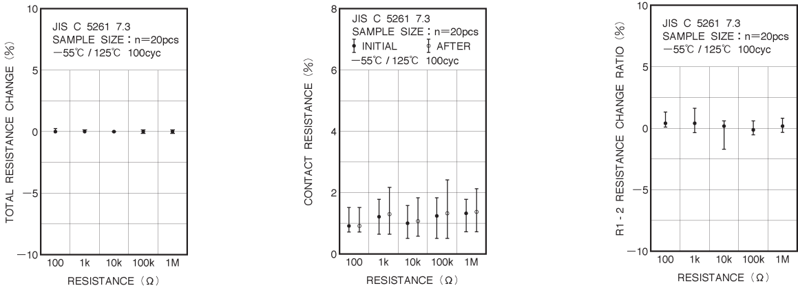
Fig.9 Temperature cycling
