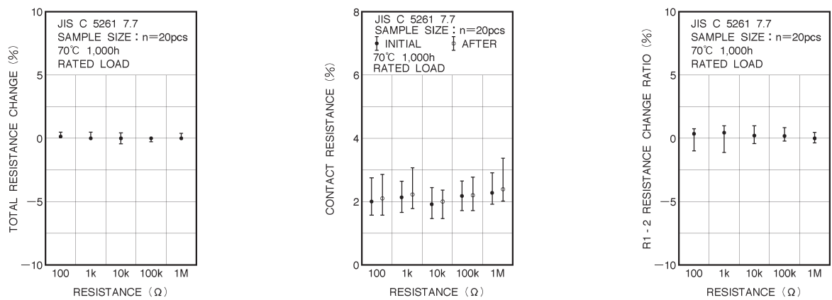
Fig.12 Endurance (rated load)
