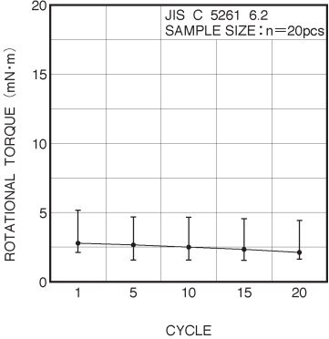
Fig.6 Rotational torque
