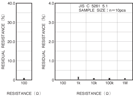
Fig.4 Residual resistance
