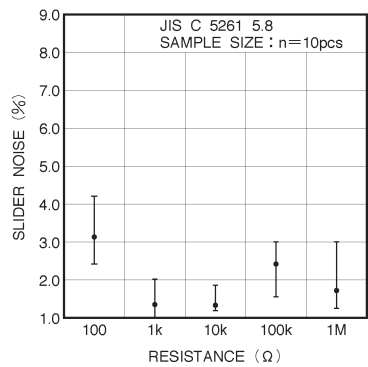
Fig.13 Wiper noise
