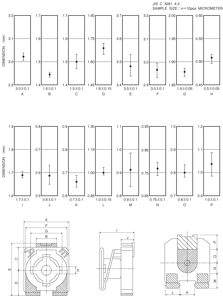
Fig.2 Dimensions
