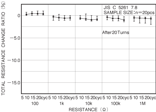
Fig.5-1 Endurance (wiper)
