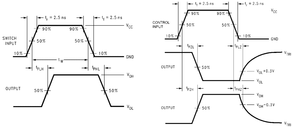
FIGURE 2. AC Waveforms
