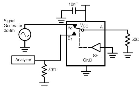
FIGURE 6. Crosstalk
