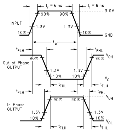
FIGURE 3. AC Waveforms
