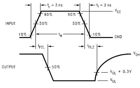
FIGURE 3. AC Waveforms
