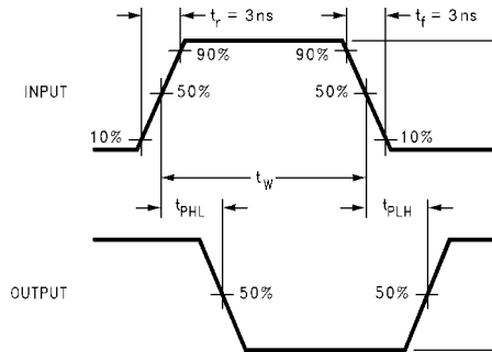
FIGURE 3. AC Waveforms
