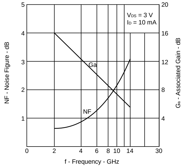
NOISE FIGURE, ASSOCIATED GAIN vs. FREQUENCY
