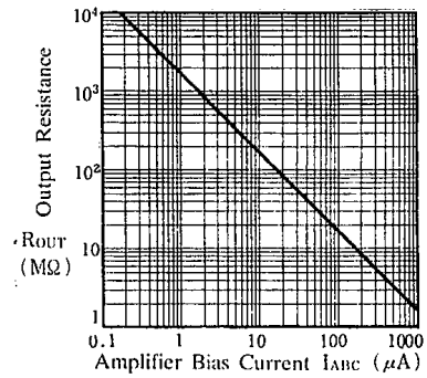
Output Resistance
