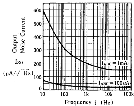
Output Noise Current vs. Frequency ( T_a = 25^\circ C )
