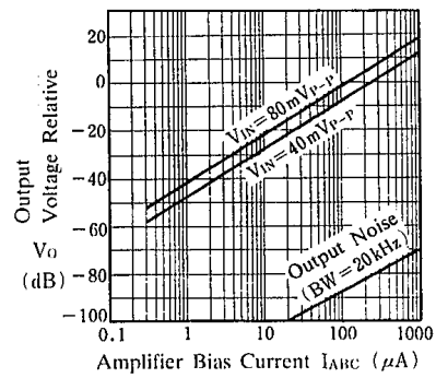
Voltage vs. Amplifier Bias Current ( V^+/V^- = \pm 15V , R_L = 10k\Omega , T_a = 25^\circ C )
