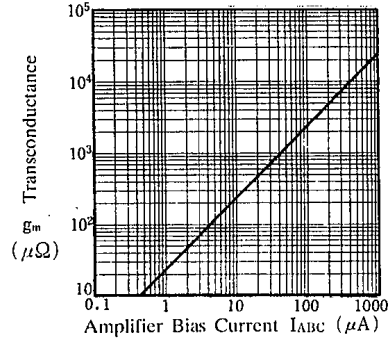
Transconductance
