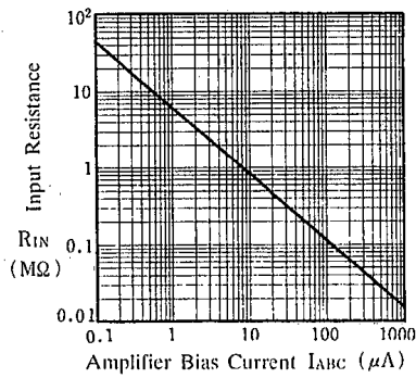
Input Resistance
