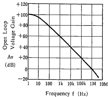
Open Loop Frequency Response ( V^+/V^- = \pm 15V , T_a = 25^\circ C )
