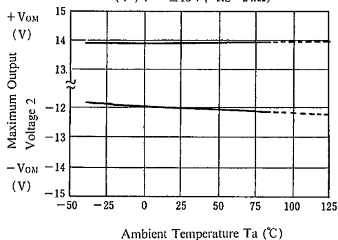
Maximum Output Voltage 2 vs. Temperature ( V^+/V^- = \pm 15\text{ V} , R_L = 2\text{ k}\Omega )
