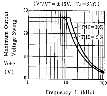
Maximum Output Voltage Swing vs. Frequency ( V^+/V^- = \pm 15V , T_a = 25^\circ C )
