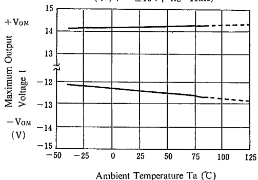
Maximum Output Voltage 1 vs. Temperature ( V^+/V^- = \pm 15\text{ V} , R_L = 10\text{ k}\Omega )
