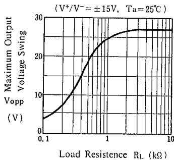
Maximum Output Voltage Swing vs. Load Resistance ( V^+/V^- = \pm 15V , T_a = 25^\circ C )
