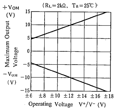
Maximum Output Voltage Swing vs. Operating Voltage ( R_L = 2k\Omega , T_a = 25^\circ C )
