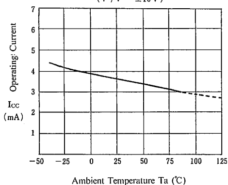
Operating Current vs. Temperature ( V^+/V^- = \pm 15\text{ V} )
