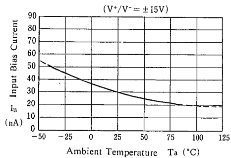
Input Bias Current vs. Temperature ( V^+/V^- = \pm 15V )
