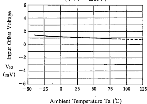
Input Offset Voltage vs. Temperature ( V^+/V^- = \pm 15\text{ V} )
