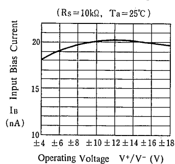
Input Bias Current vs. Operating Voltage ( R_s = 10k\Omega , T_a = 25^\circ C )
