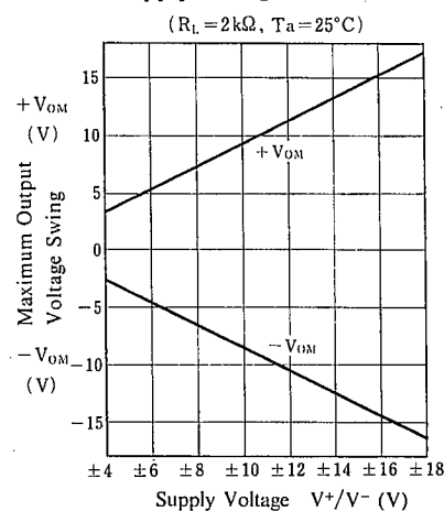
Maximum Output Voltage Swing vs. Supply Voltage
