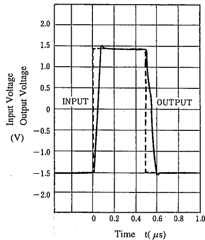
Pulse Response
