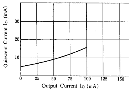
NJM2930F05 Output Current vs. Quiescent Current
