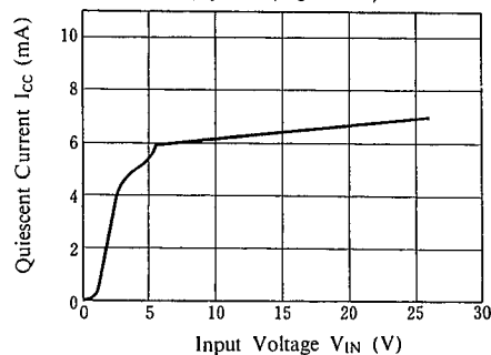
NJM2930F05/L05 I_{CC}-V_{IN}
