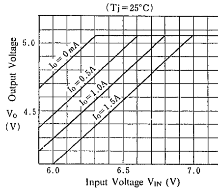
NJM7812 Dropout Characteristics
