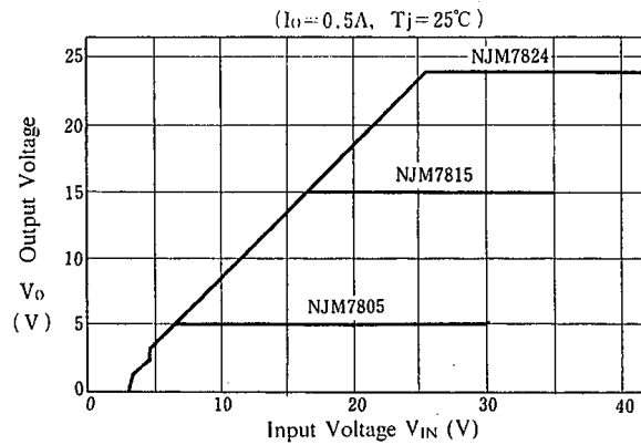
NJM7805 Dropout Characteristics
