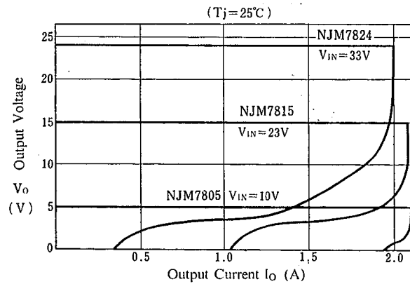
NJM7805/15/24 Load Characteristics
