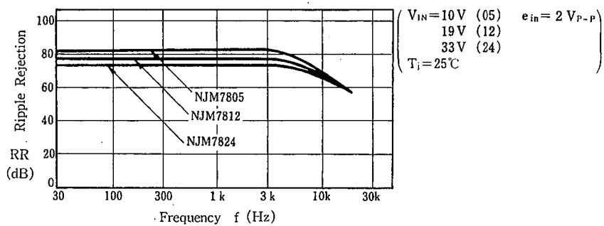
NJM7805/12/24 Ripple Rejection vs. Frequency
