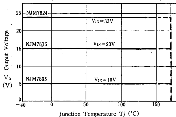
NJM7805/15/24 Output Voltage vs. Junction Temperature
