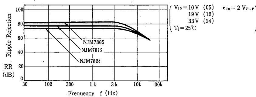
NJM7805/12/24 Ripple Rejection vs. Frequency
