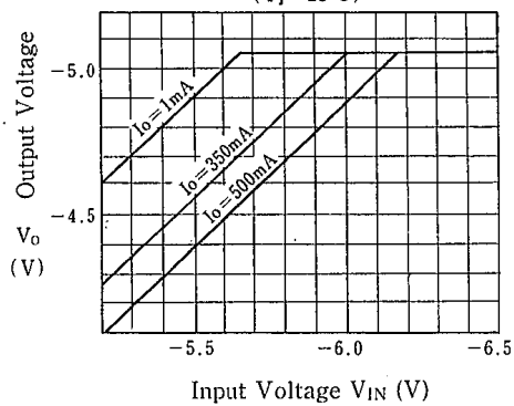
NJM79M05 Dropout Characteristics
