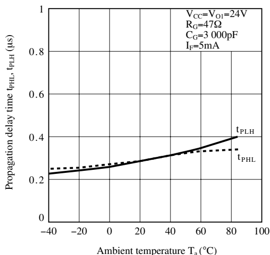
Fig.27 Propagation Delay Time vs. Ambient Temperature
