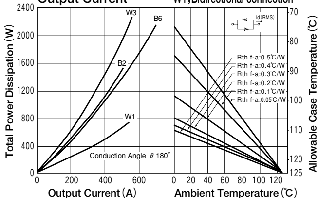
Output Current
