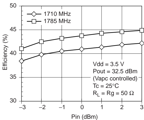
Efficiency vs Pin
