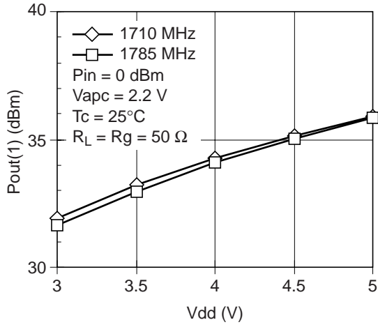
Pout(1) vs Vdd
