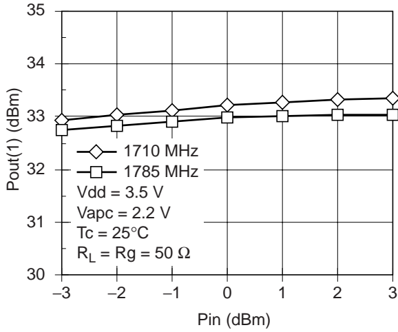
Pout(1) vs Pin
