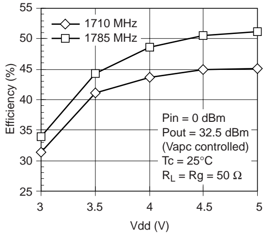
Efficiency vs Vdd
