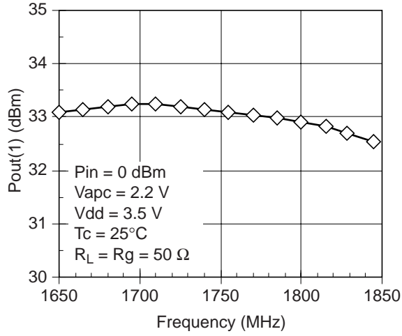
Pout(1) vs Frequency
