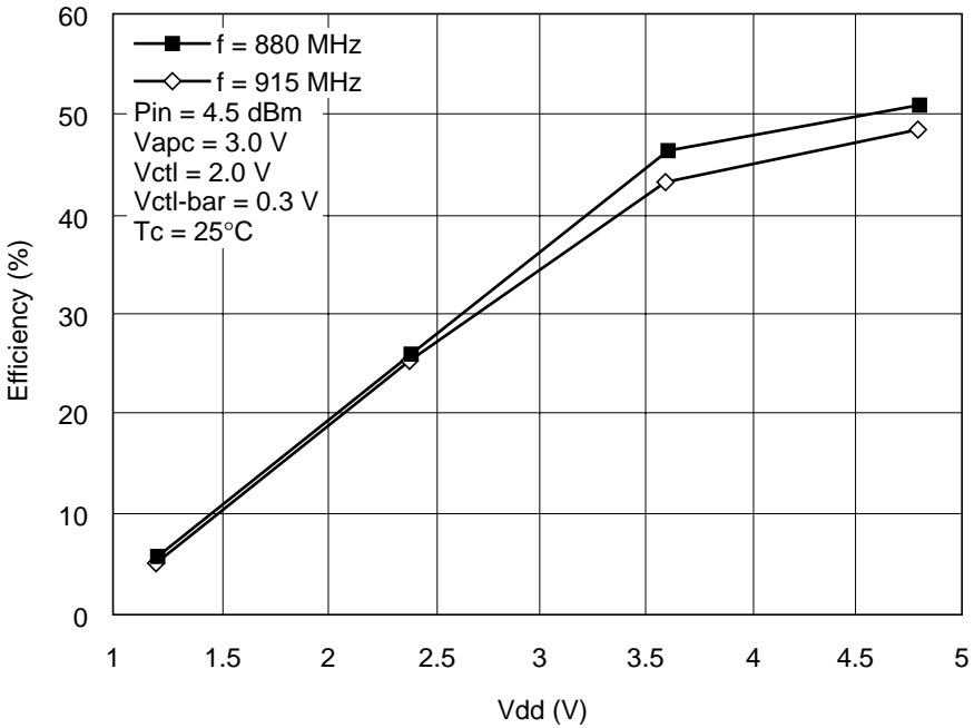
GSM mode Eff-Vdd curve
