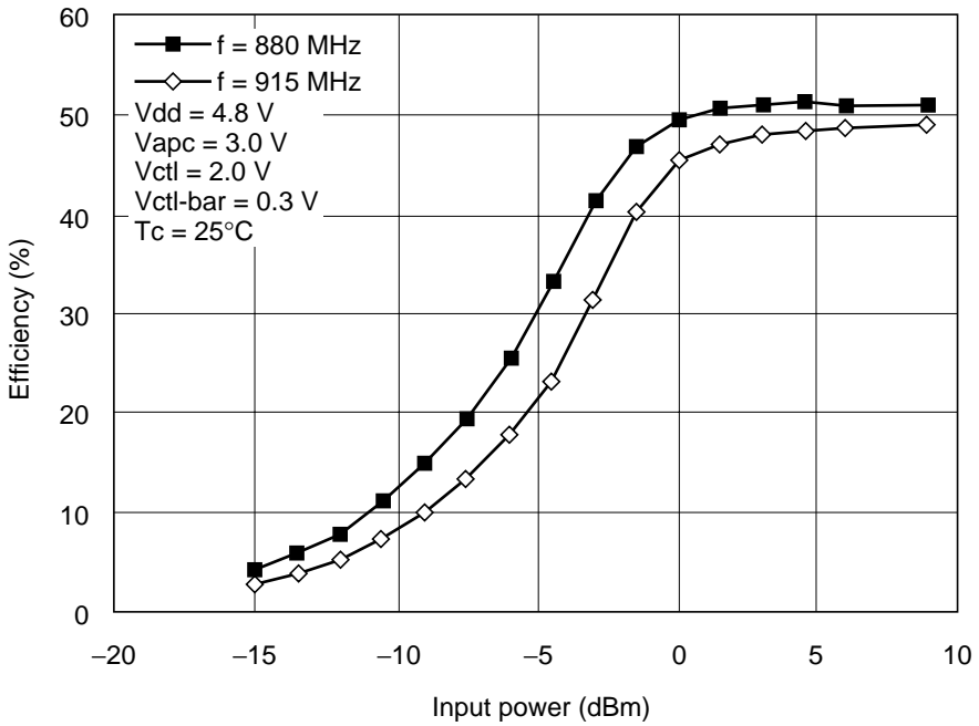
GSM mode Eff-pin curve
