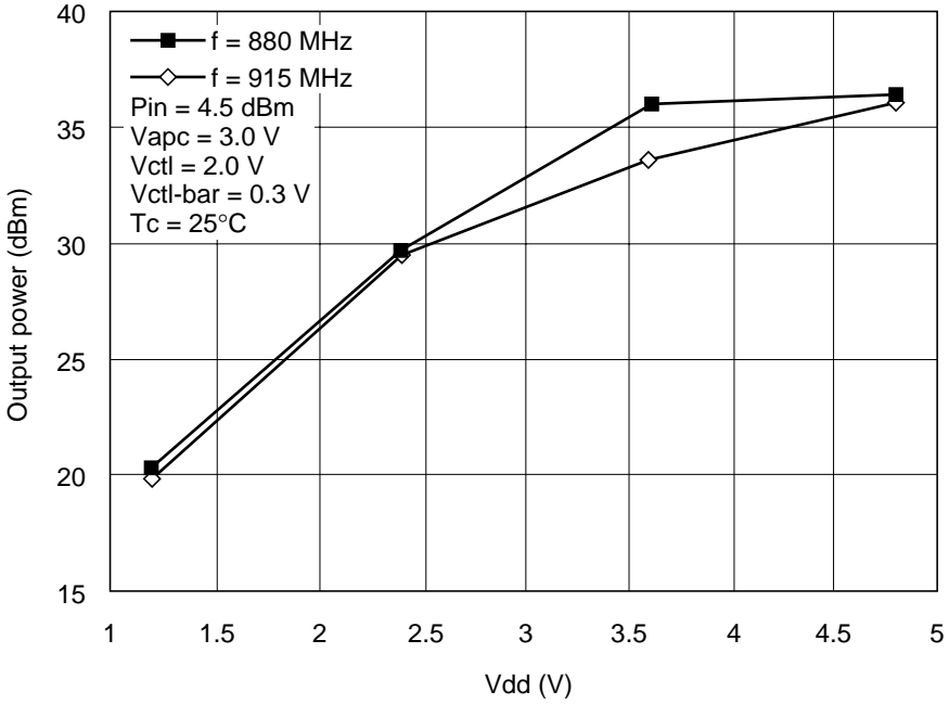
GSM mode Po-Vdd curve
