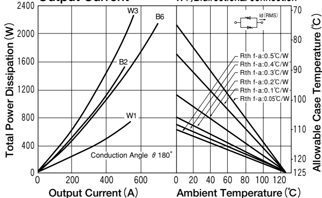
Output Current
