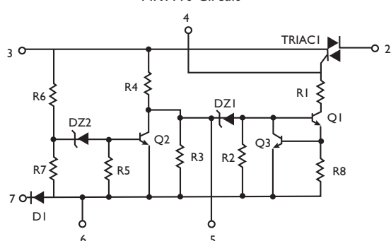
MK1110 Circuit
