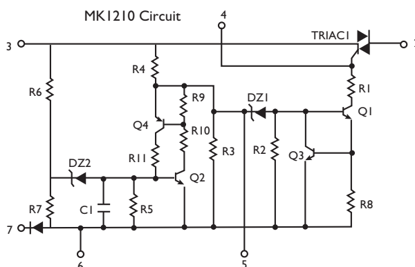
MK1210 Circuit
