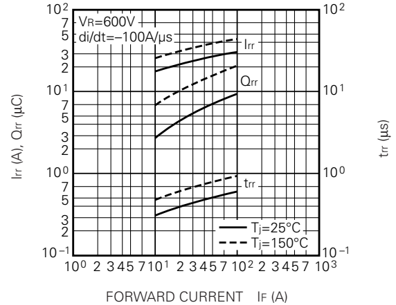
REVERSE RECOVERY CHARACTERISTICS (VS. I_F ) (TYPICAL)
