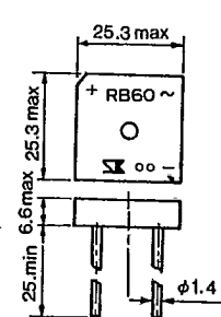
Outline Drawing ㉓
