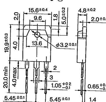
Outline Drawing ⑳
