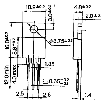
Outline Drawing ⑲
