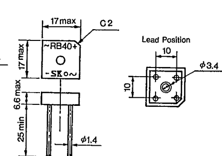
Outline Drawing ㉔
