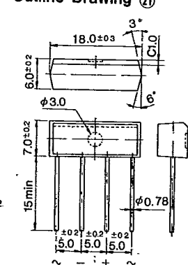
Outline Drawing ㉑
