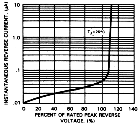
FIG.4-TYPICAL REVERSE CHARACTERISTICS
