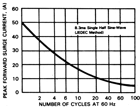
FIG.1-MAXIMUM NON-REPETITIVE PEAK
