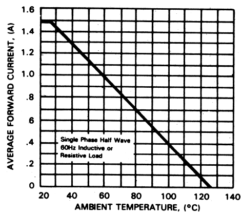
FIG.2-TYPICAL FORWARD CURRENT
