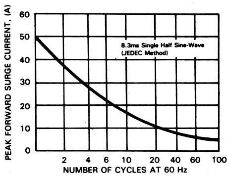
FIG.1-MAXIMUM NON-REPETITIVE PEAK
