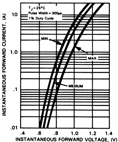
FIG.3-TYPICAL INSTANTANEOUS FORWARD
